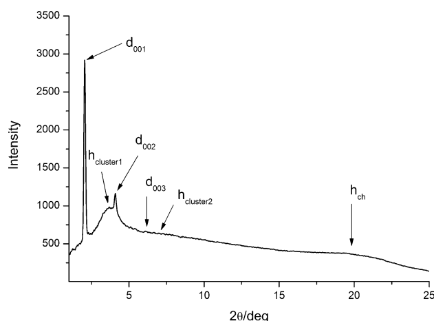
Figure 2. X-ray powder diffraction pattern for compound WL 2 at 60 °C ( \lambda = 1.54 \text{ \AA} ).
