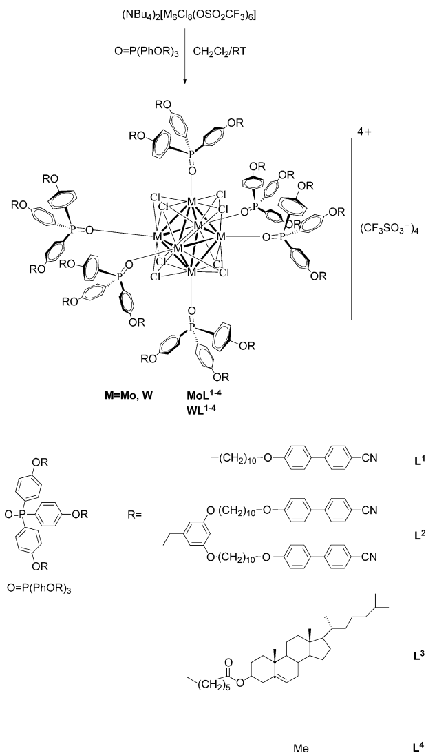
Scheme 1. Preparation of new hexa-functionalized \text{Mo}_6 and \text{W}_6 clusters.
